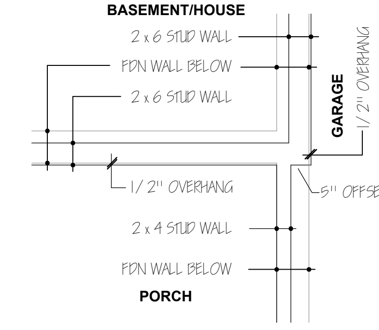
2 DET @ GARAGE STUD WALL SCALE: 1/2" = 1'-0"
