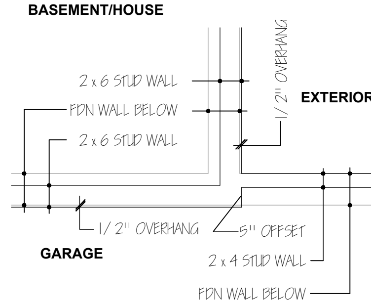
1 DET @ GARAGE STUD WALL SCALE: 1/2" = 1'-0"
