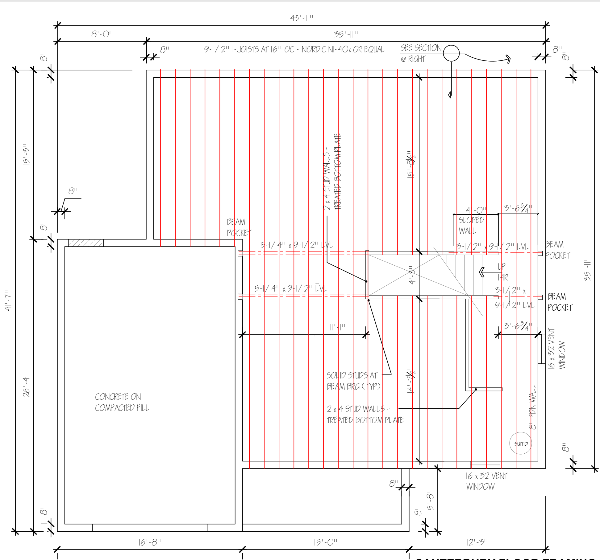
CANTERBURY FLOOR FRAMING SCALE: 3/16" = 1'-0"
